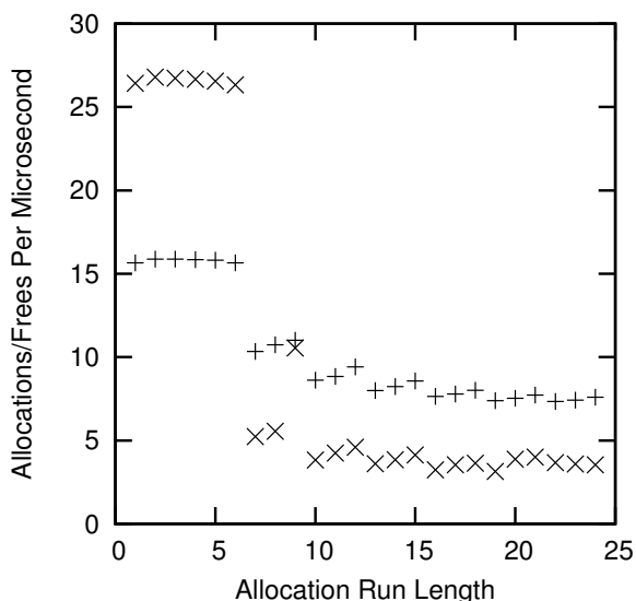
Figure 5.31: Allocator Cache Performance
