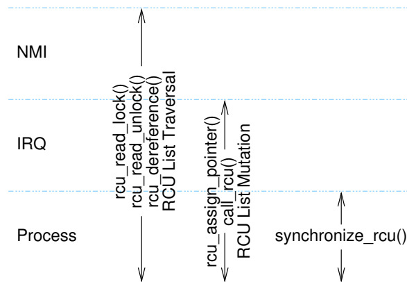
Figure 8.32: RCU API Usage Constraints
