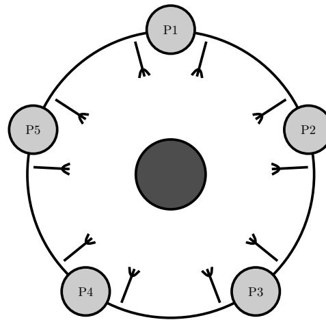
Figure G.3: Dining Philosophers Problem, Fully Partitioned
