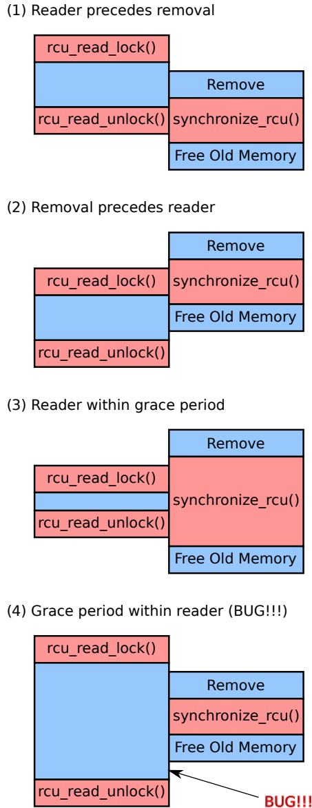
Figure 9.14: Summary of RCU Grace-Period Ordering Guarantees
