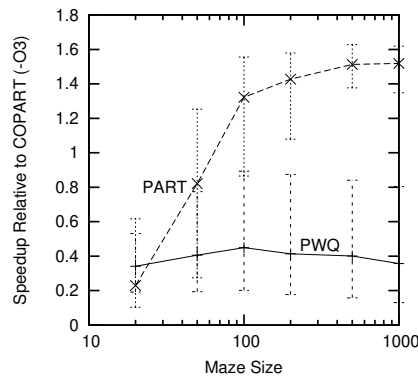
Figure 6.32: Varying Maze Size vs. COPART
