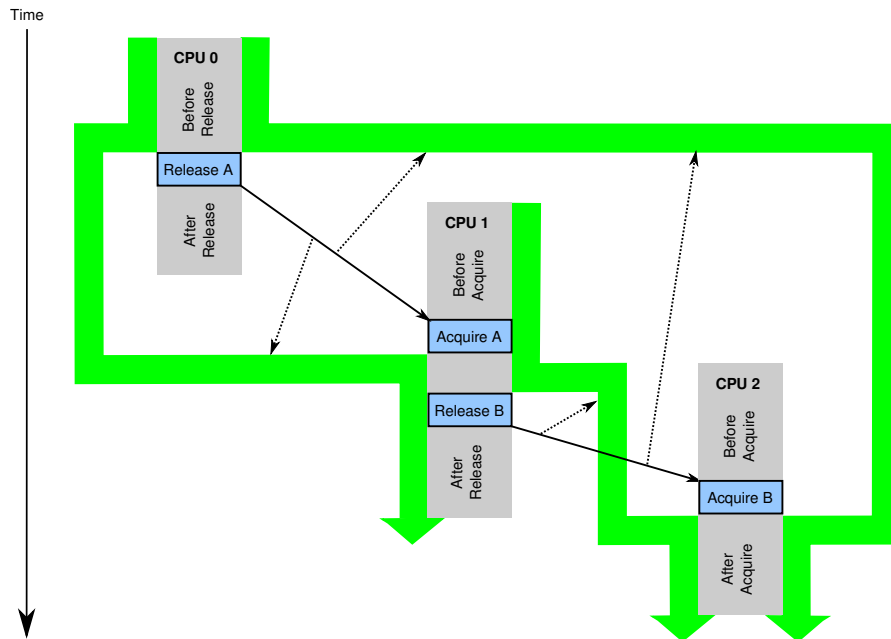
Figure 15.25: Release-Acquire Intuitions
