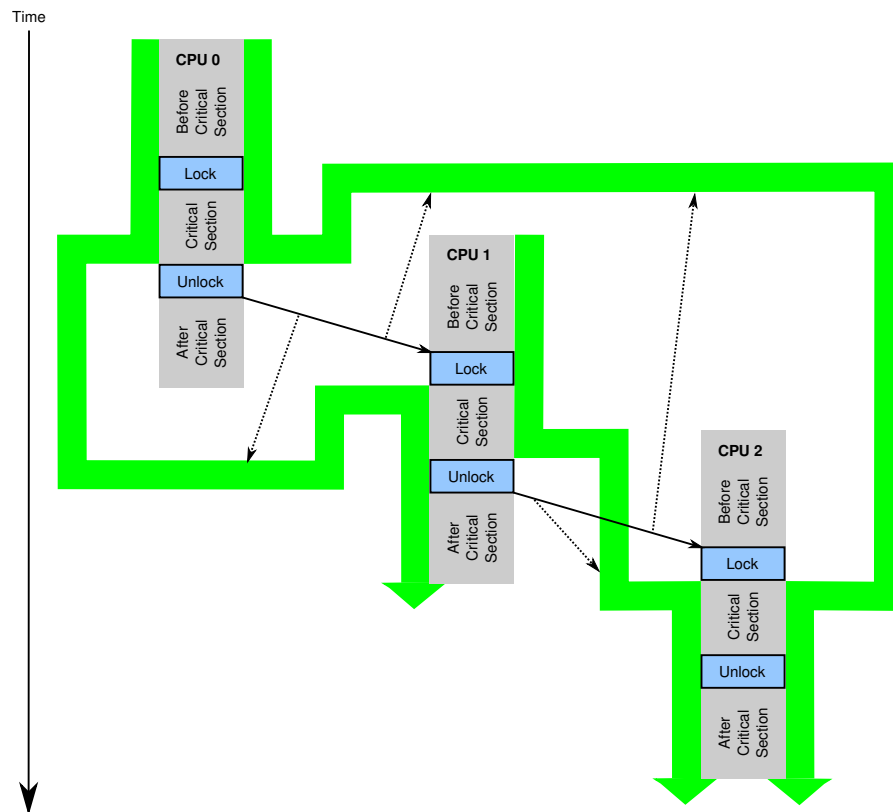
Figure 15.24: Locking Intuitions
