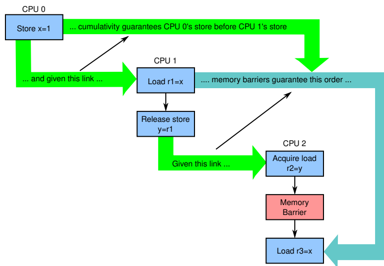
Figure 15.11: Cumulativeness
