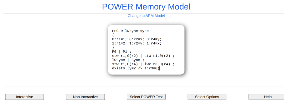
Figure 15.15: PPCMEM Initial R State
