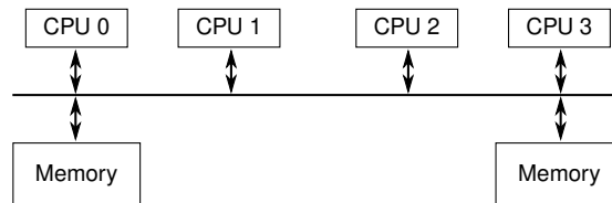
Figure 15.9: Global System Bus And Multi-Copy Atomicity
