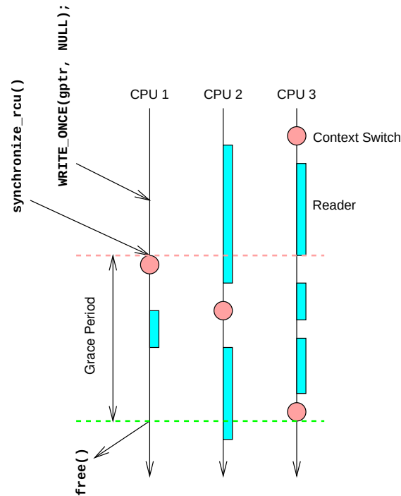
Figure 9.8: QSBP: Waiting for Pre-Existing Readers
