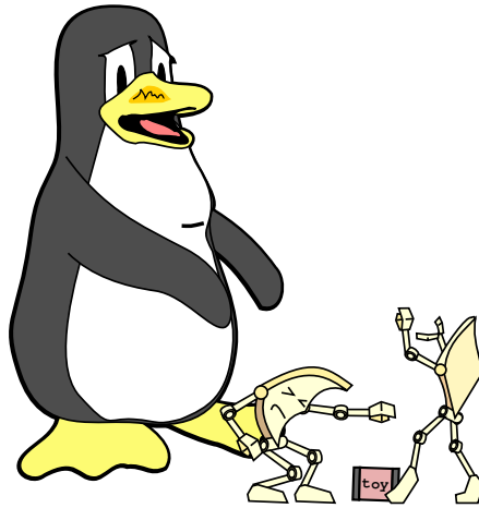
Figure 6.13: Lock Contention
