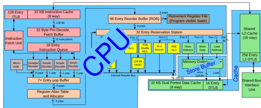
Figure 15.2: Intel Core 2 Architecture Simplified
