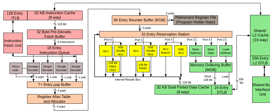
Figure 15.1: Intel Core 2 Architecture
