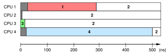
Figure 15.6: A Variable With Multiple Simultaneous Values
