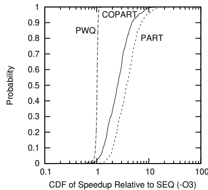
Figure 6.30: Partitioned Coroutines
