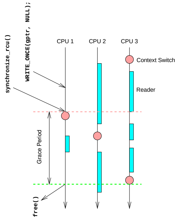
Figure 9.8: QSB: Waiting for Pre-Existing Readers
