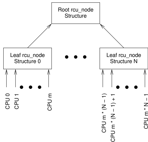
Figure 7.10: Locking Hierarchy
