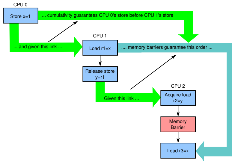
Figure 15.9: Cumulativity
