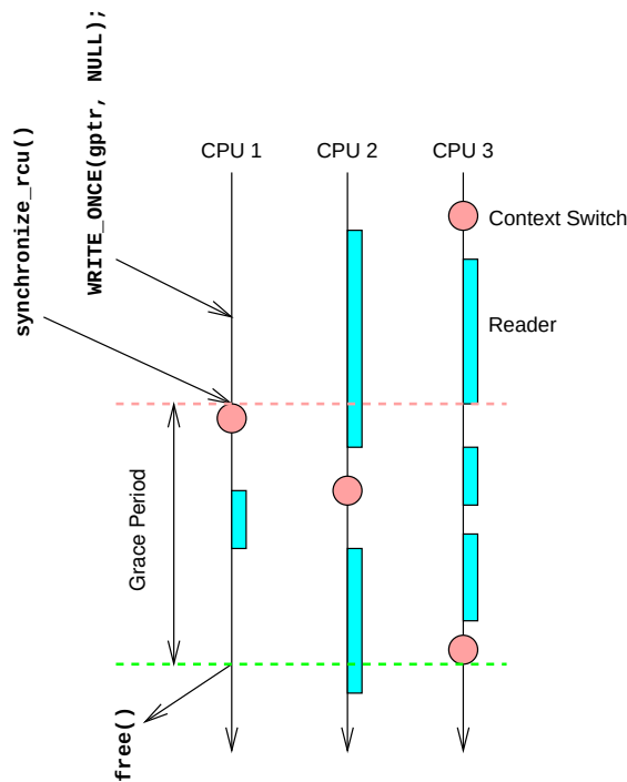
Figure 9.8: QSB: Waiting for Pre-Existing Readers
