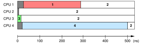
Figure 15.9: A Variable With Multiple Simultaneous Values
