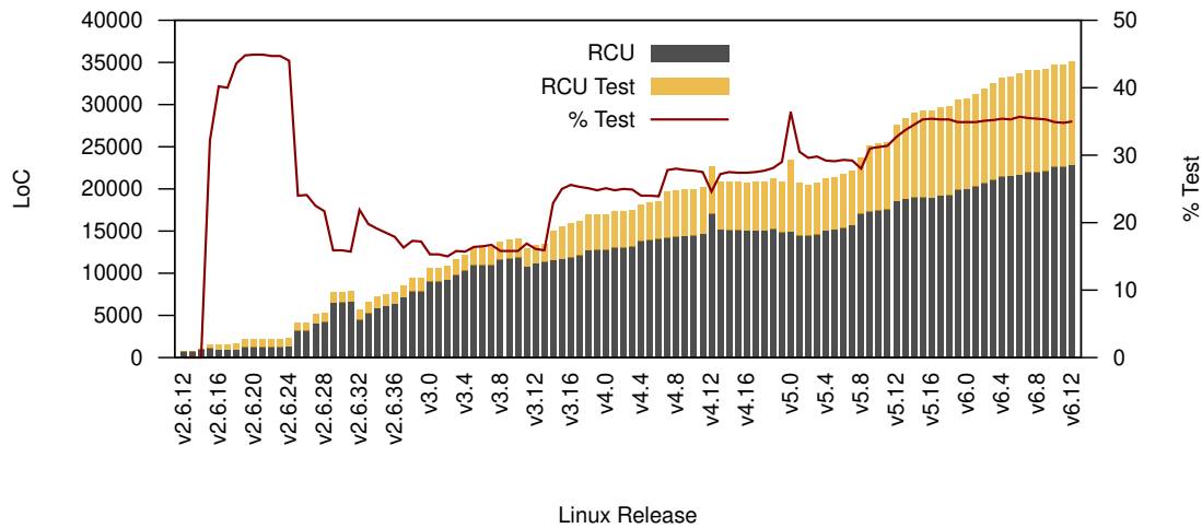
Figure 12.4: Linux-Kernel RCU Test Code
