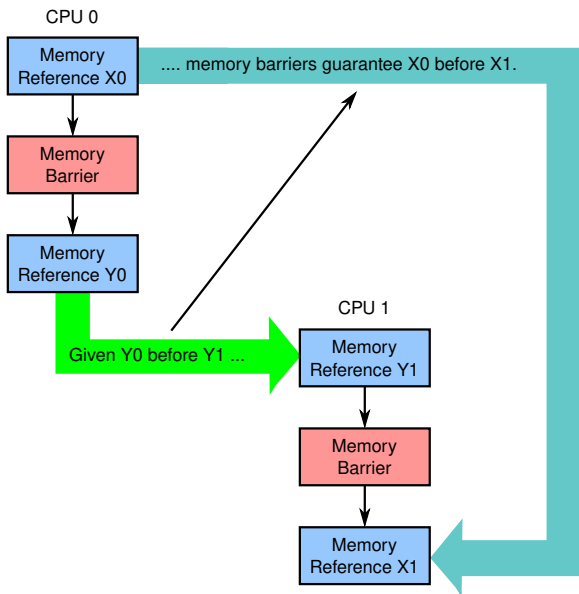
Figure 15.8: Memory Barriers Provide Conditional If-Then Ordering
