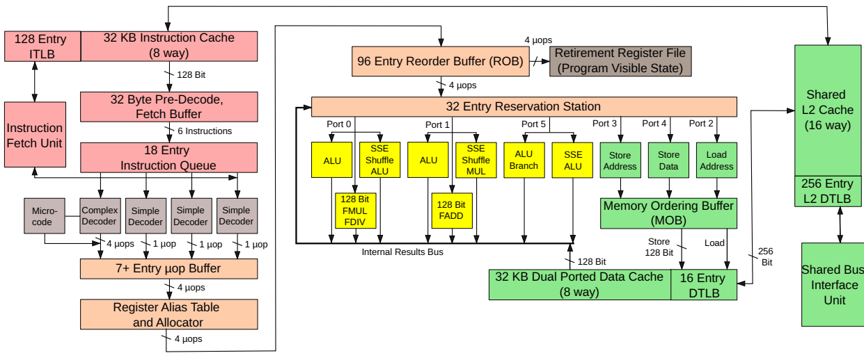
Figure 15.4: Intel Core 2 Architecture
