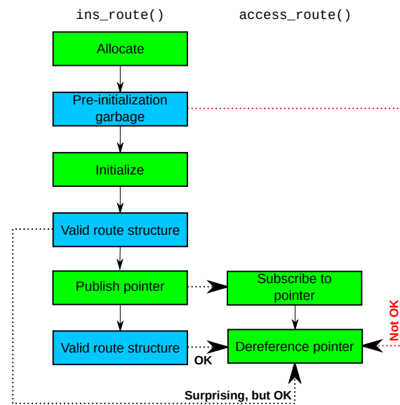
Figure 9.10: Publication/Subscription Constraints
